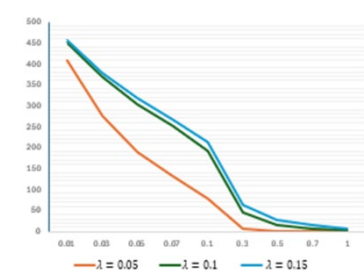
(c) SARFIMA(1, 0, 0)(1, 0.4, 0) 12
