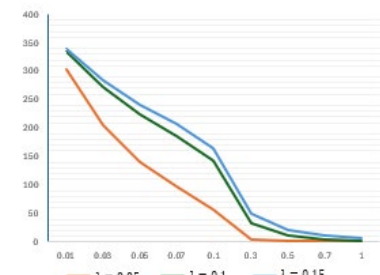
(c) SARFIMA(1, 0, 0)(1, 0.4, 0) 12
