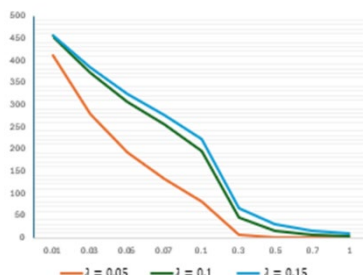
(a) SARFIMA(1, 0, 0)(1, 0.1, 0) 12
