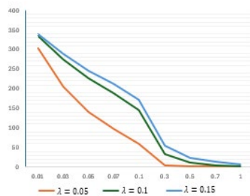
(a) SARFIMA(1, 0, 0)(1, 0.1, 0) 12
