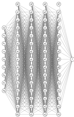
7(c) FNN-Large
