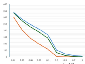
(b) SARFIMA(1, 0, 0)(1, 0.2, 0) 12
