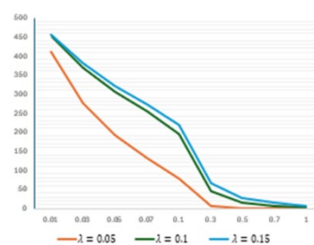
(b) SARFIMA(1, 0, 0)(1, 0.2, 0) 12
